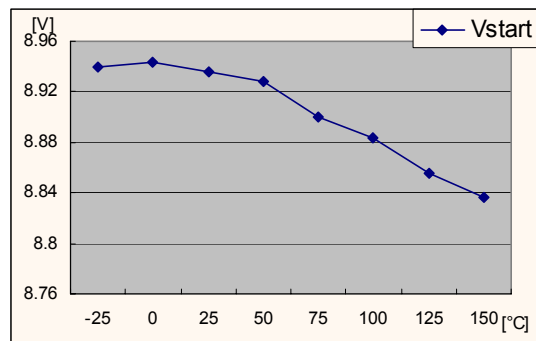
Figure 2. Start Threshold Voltage
