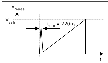
Figure 15 Leading Edge Blanking
