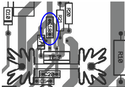
Figure 56B Detail X, Soft Start Capacitor C 18 Layout Recommendation
