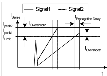
Figure 16 Current Limiting
