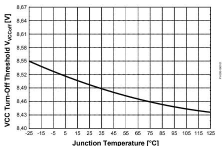
Figure 31 VCC Turn-Off Threshold V_{VCCoff} vs. T_j
