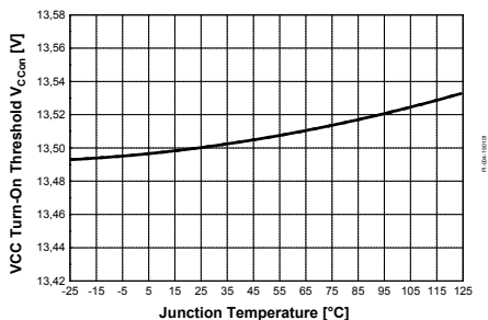
Figure 30 VCC Turn-On Threshold V_{VCCon} vs. T_j
