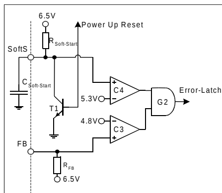
Figure 21 FB-Detection
