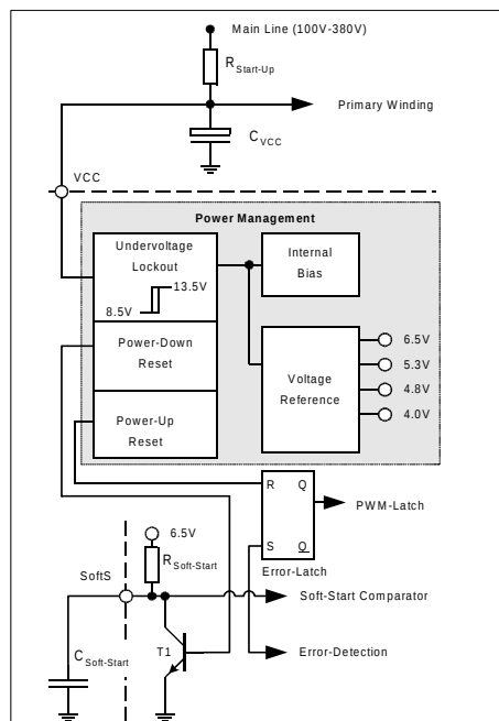
Figure 5 Power Management
