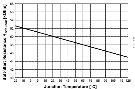
Figure 43 Soft-Start Resistance R_{Soft-Start} vs. T_J
