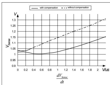
Figure 18 Overcurrent Shutdown
