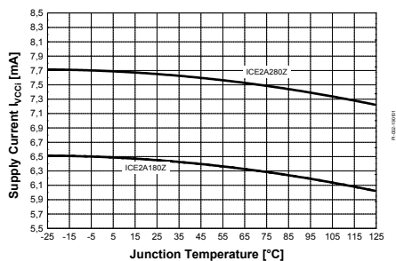
Figure 28 Supply Current I_{VCC1} vs. T_j
