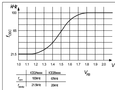
Figure 14 Frequency Dependence
