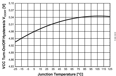
Figure 32 VCC Turn-On/Off Hysteresis V_{VCHY} vs. T_j
