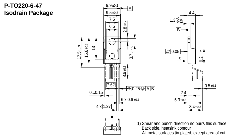
Figure 60 P-TO220-6-47 (Isodrain Package)
