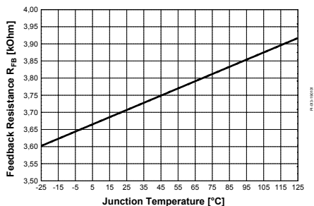
Figure 42 Feedback Resistance R_{FB} vs. T_J
