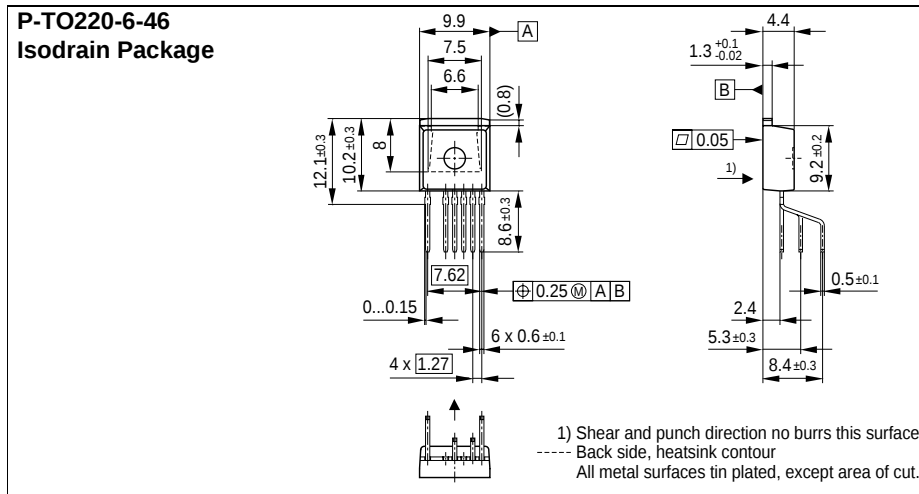
Figure 59 P-TO220-6-46 (Isodrain Package)
