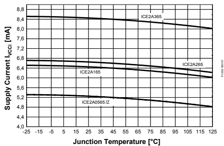
Figure 26 Supply Current I_{VCC1} vs. T_j
