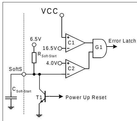
Figure 23 Overvoltage Detection
