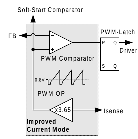
Figure 6 Current Mode
