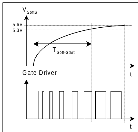
Figure 11 Soft-Start Phase
