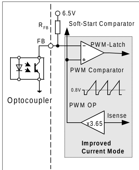
Figure 10 PWM Controlling
