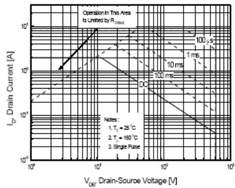
Figure 9-2. Maximum Safe Operating Area for TSF2N60M
