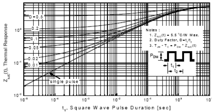
Figure 11-2. Transient Thermal Response Curve for TSF2N60M
