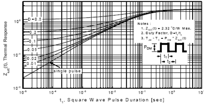
Figure 11-1. Transient Thermal Response Curve for TSP2N60M
