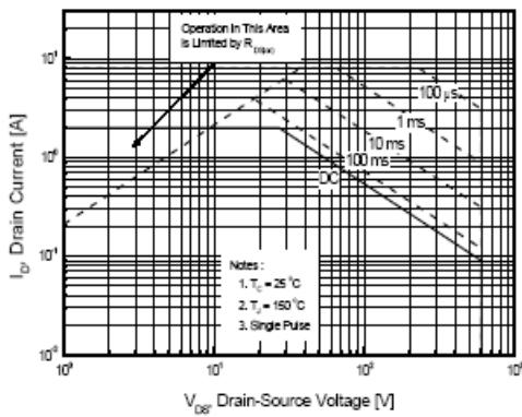
Figure 9-1. Maximum Safe Operating Area for TSP2N60M
