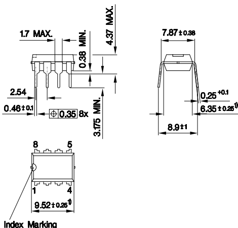
Figure 21 PG-DIP-8-6 (Leadfree Plastic Dual In-Line Outline)
