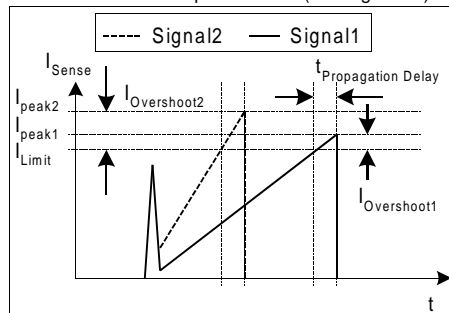
Figure 12 Current Limiting
