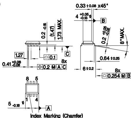
Figure 22 P-DSO-8-8 (Plastic Dual Small Outline)
