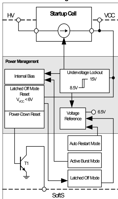
Figure 4 Power Management
