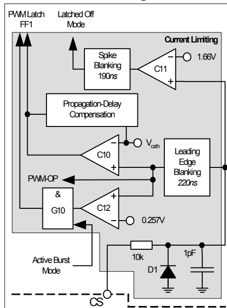
Figure 10 Current Limiting
