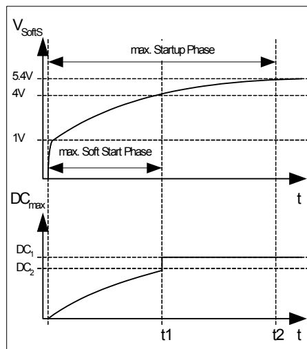
Figure 6 Startup Phase
